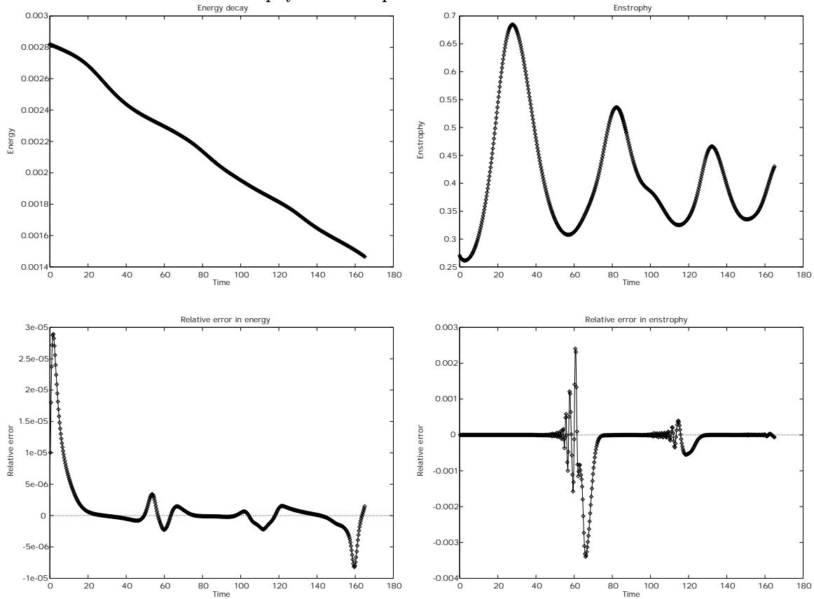
Figure 4: Top: Evolution of energy and enstrophy for Figure 3 . Bottom: Relative errors in \frac{dE}{dt} and \frac{d\Omega}{dt} for Figure 3 where the exact solution was calculated using right hand sides of (23) and (24) and the approximate solution was computed by using a leapfrog scheme after calculating E and \Omega at t - \delta t and t + \delta t .
