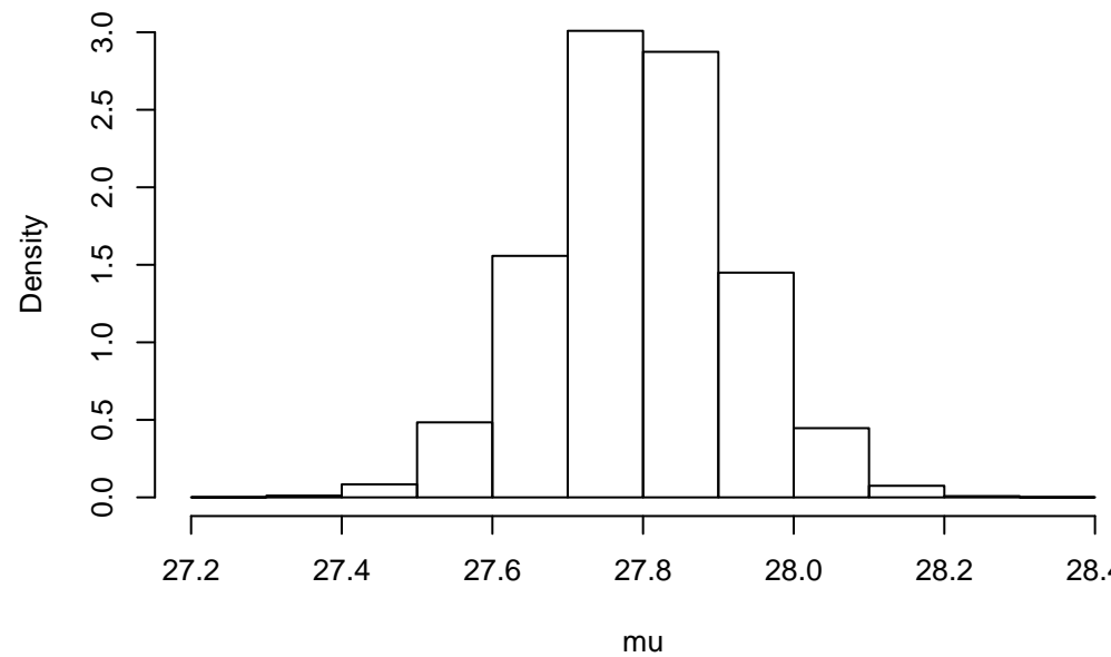
Histogram of draws3[(101:10000), 1]
