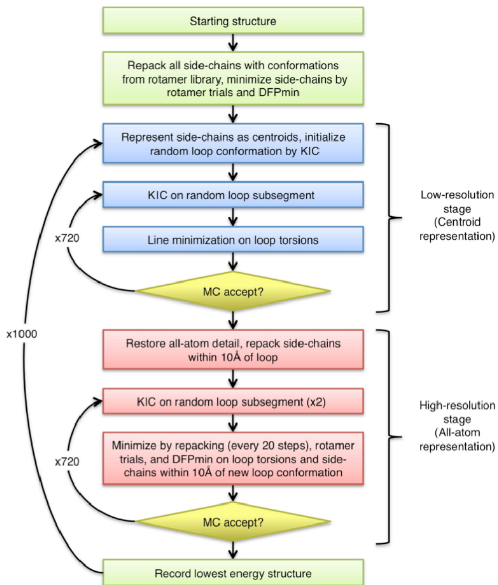
Supplementary Figure 2 – The Rosetta KIC loop reconstruction protocol.
