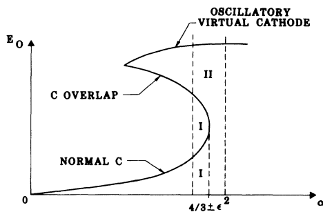
FIG. 5. Electric field at the injection plane vs current \alpha for I=0 . Plot depicts the normal C-flow (stable) and C-overlap (unstable) solutions. Oscillating virtual-cathode (stable) solution is also shown. Regions I and II define the domains of attraction of the normal-C and virtual-cathode solutions near the SCL, \alpha = \frac{4}{3} .
