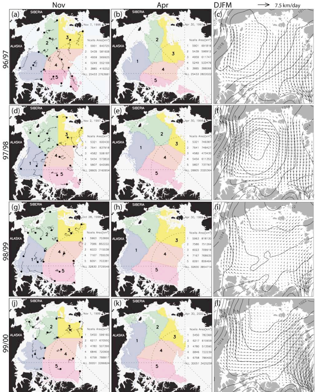
Figure 2. Net deformation of the ice cover between November and April and the mean DJFM ice motion. (a-c) 96/97. (d-f) 97/98. (g-i) 98/99. (j-l) 99-00. Solid circles (•) mark the initial location of select RGPS ice motion trajectories in (a), (d), (g), and (j). Mean sea-level pressure distributions during the period are contoured. (Isobar intervals: 2 hPa)
