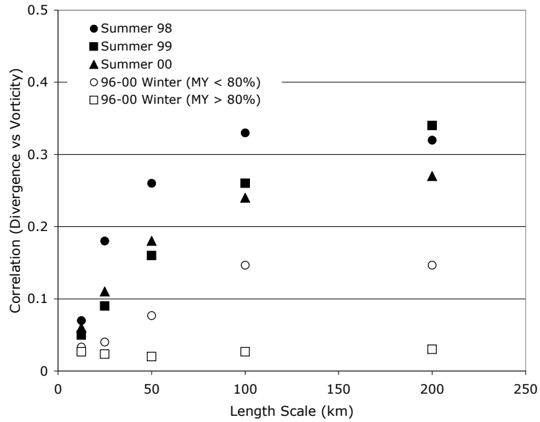
Figure 8. Seasonal and regional correlations between divergence and vorticity at different length scales. The significance of the reported correlations is all at the 0.01 level.
